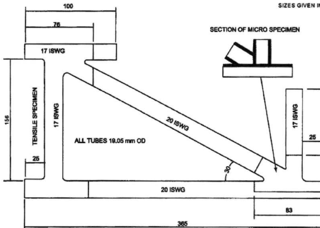
FIGURE 5 Tube to tube weld
